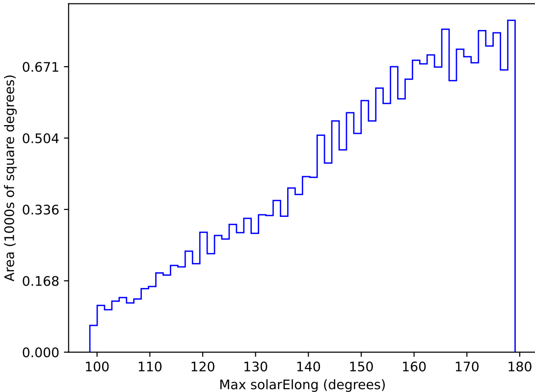
scp_reweight_v3.3_10yrs All sky y band: Max solarElong
