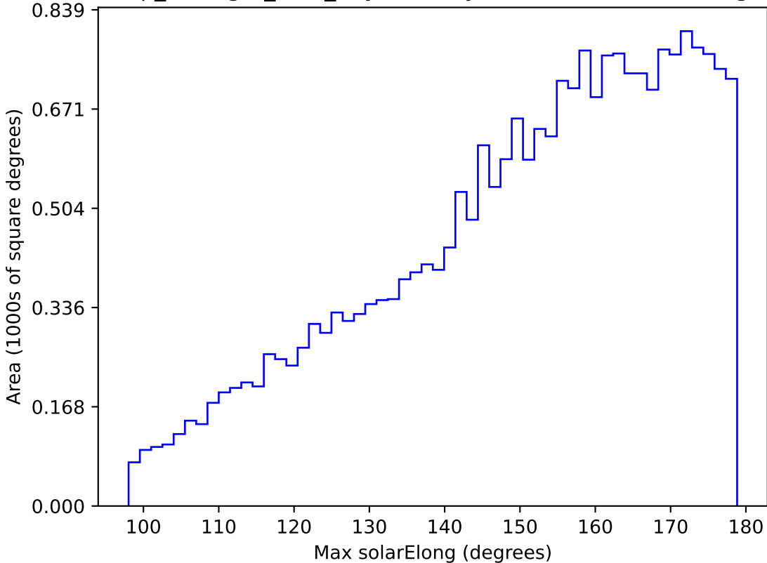
scp_reweight_v3.3_10yrs All sky u band: Max solarElong
