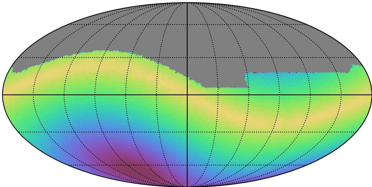
scp_reweight_v3.3_10yrs All sky r band: Max solarElong
