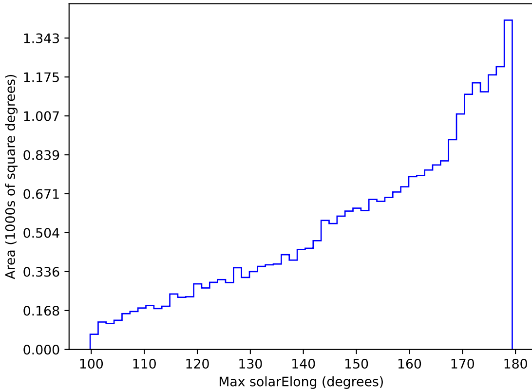
scp_reweight_v3.3_10yrs All sky r band: Max solarElong
