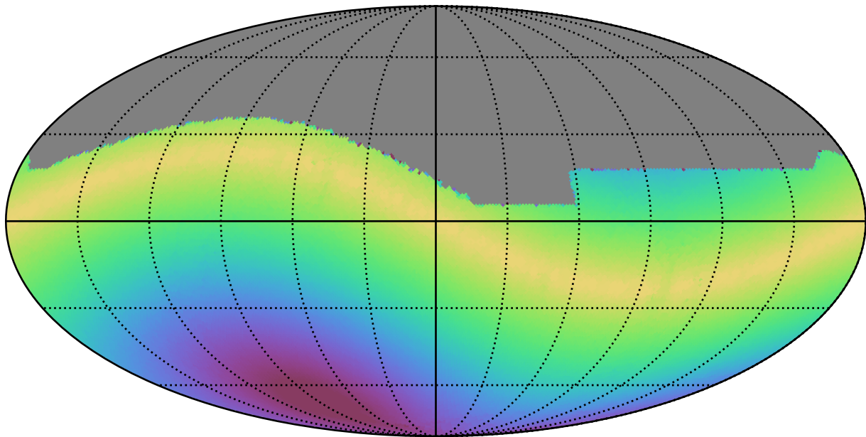
scp_reweight_v3.3_10yrs All sky i band: Max solarElong
