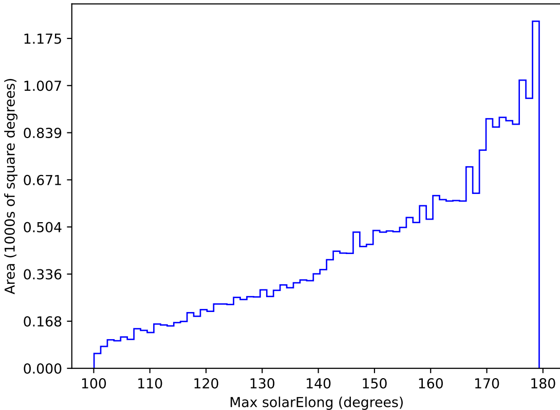
scp_reweight_v3.3_10yrs All sky i band: Max solarElong
