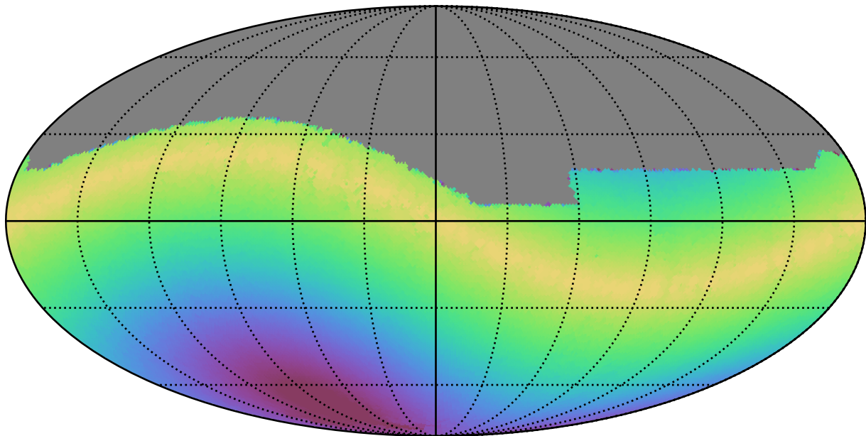
scp_reweight_v3.3_10yrs All sky g band: Max solarElong
