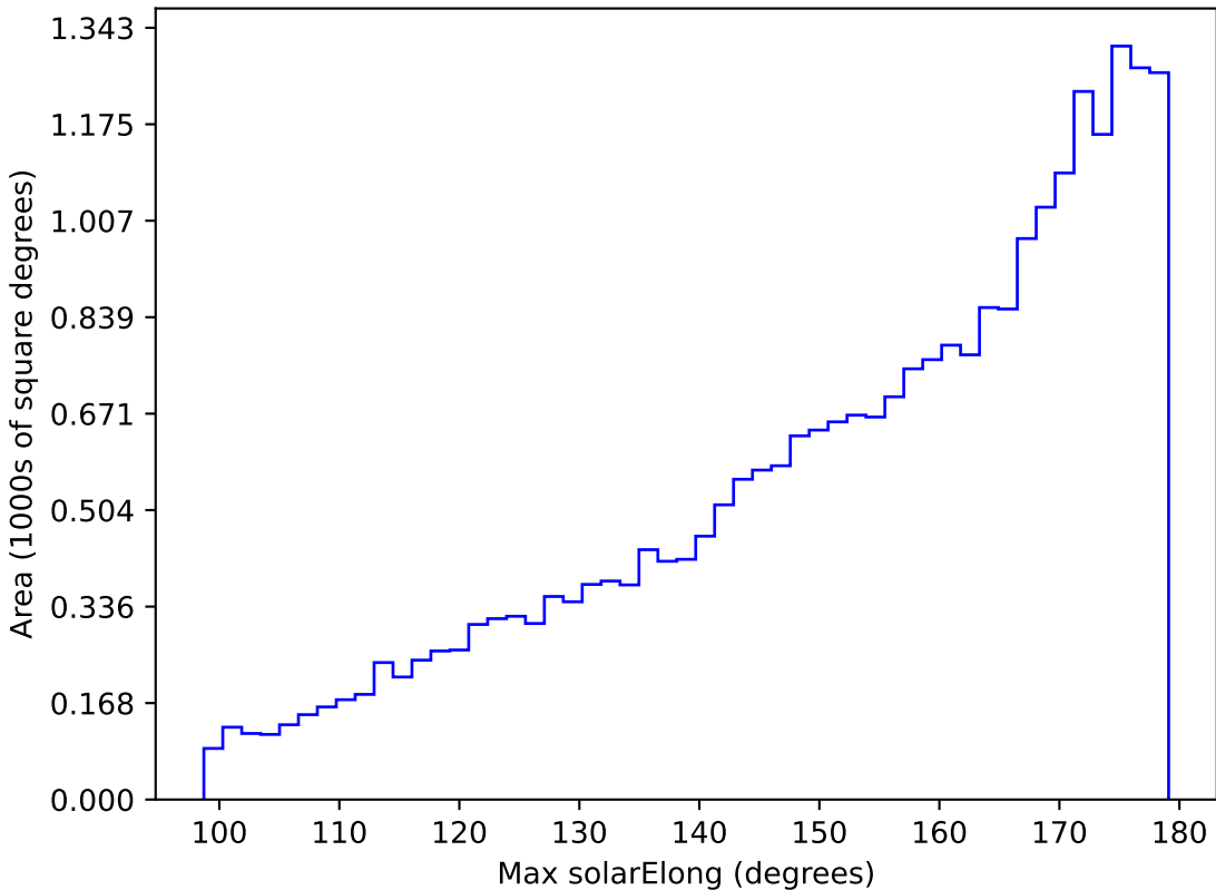
scp_reweight_v3.3_10yrs All sky g band: Max solarElong
