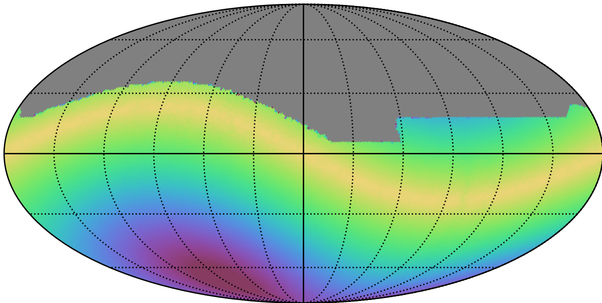
scp_reweight_v3.3_10yrs All sky all bands: Max solarElong
