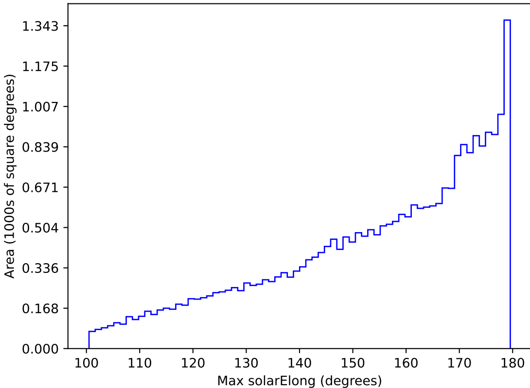
scp_reweight_v3.3_10yrs All sky all bands: Max solarElong
