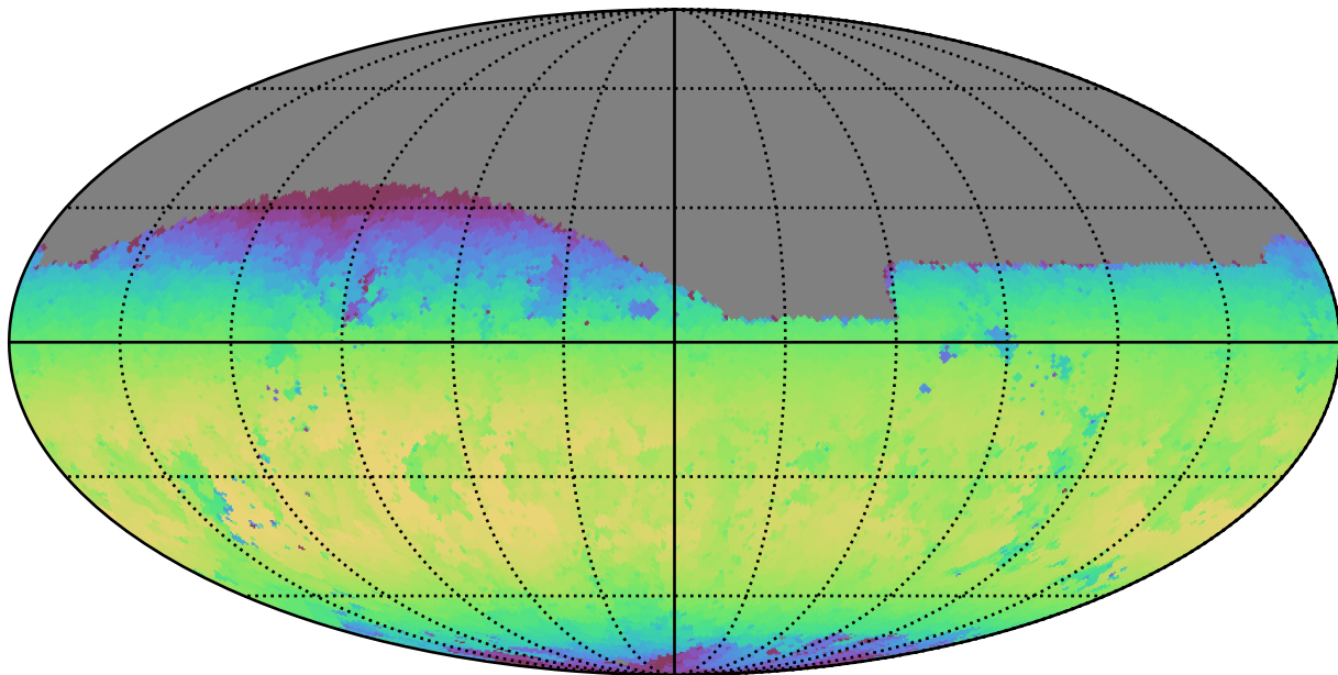
scp_reweight_v3.3_10yrs Yr 1 z band: Max skyBrightness
