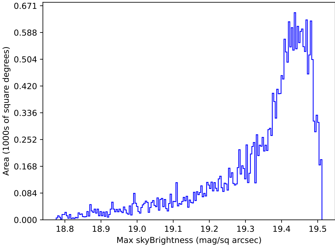
scp_reweight_v3.3_10yrs Yr 1 z band: Max skyBrightness
