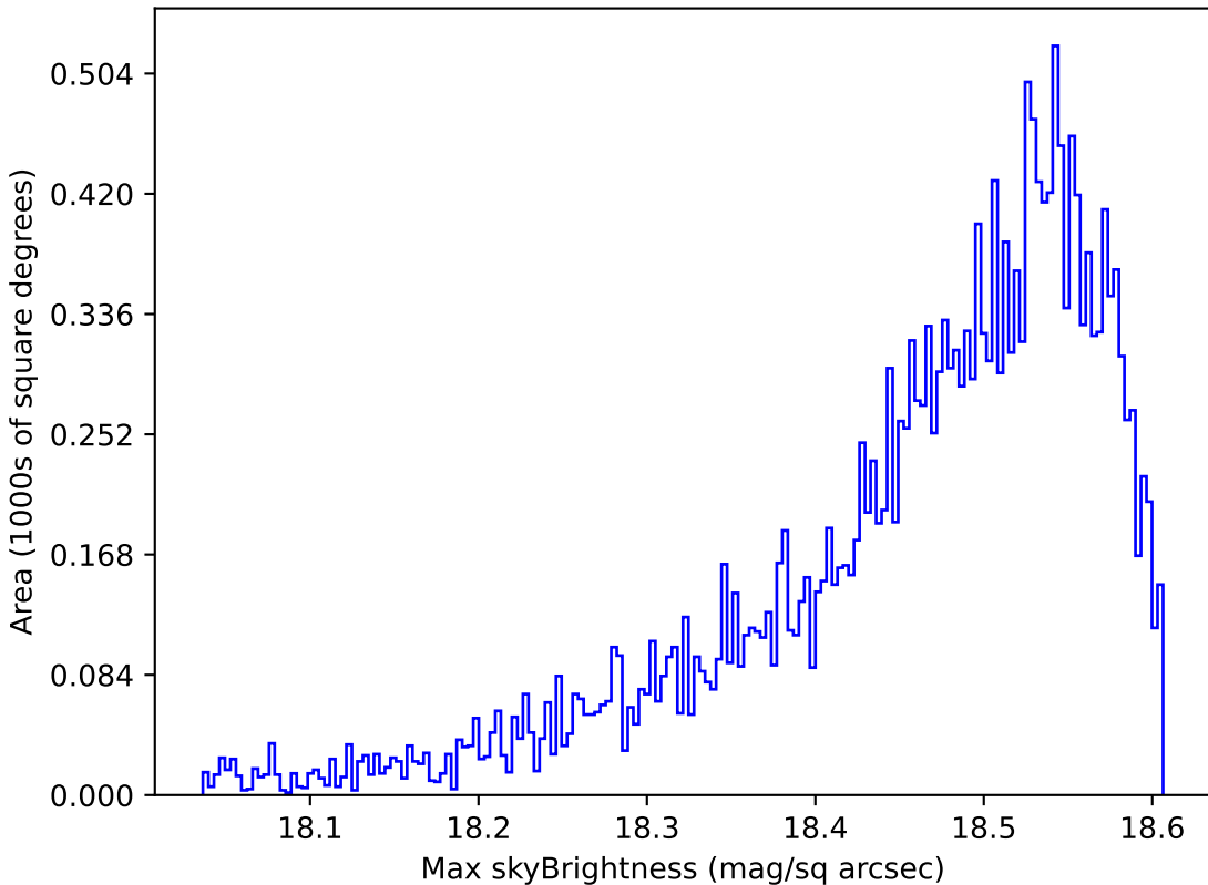
scp_reweight_v3.3_10yrs Yr 1 y band: Max skyBrightness
