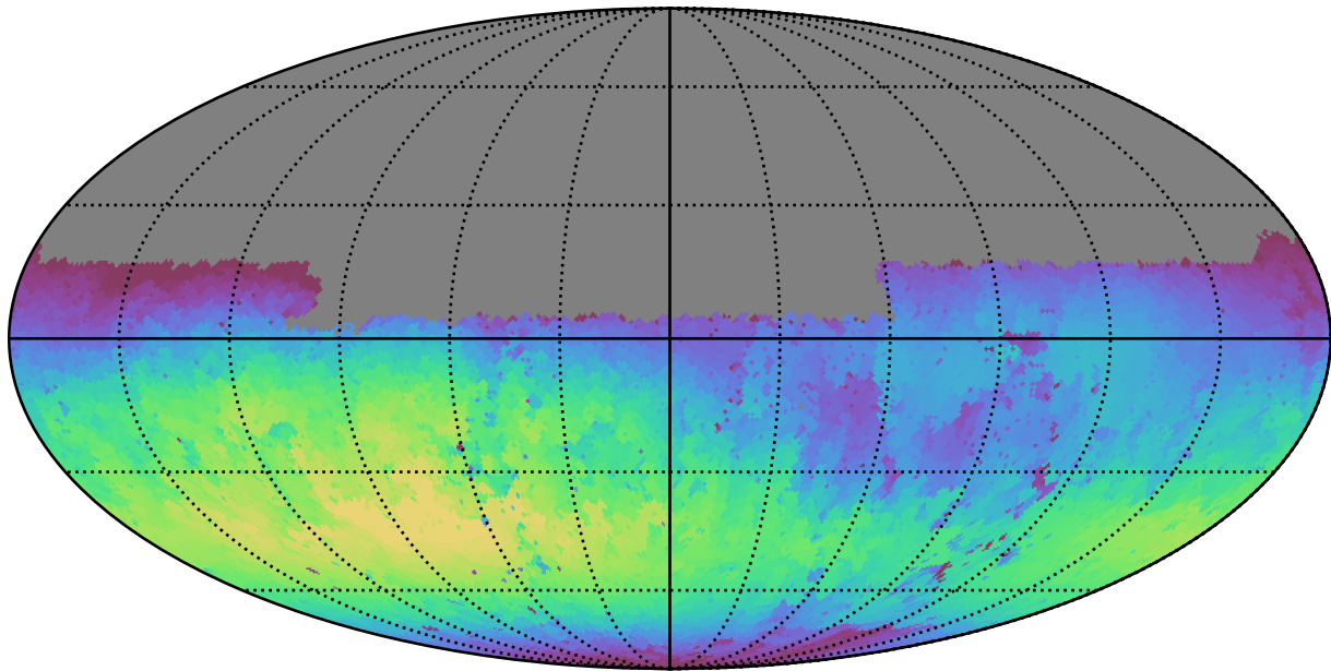
scp_reweight_v3.3_10yrs Yr 1 u band: Max skyBrightness
