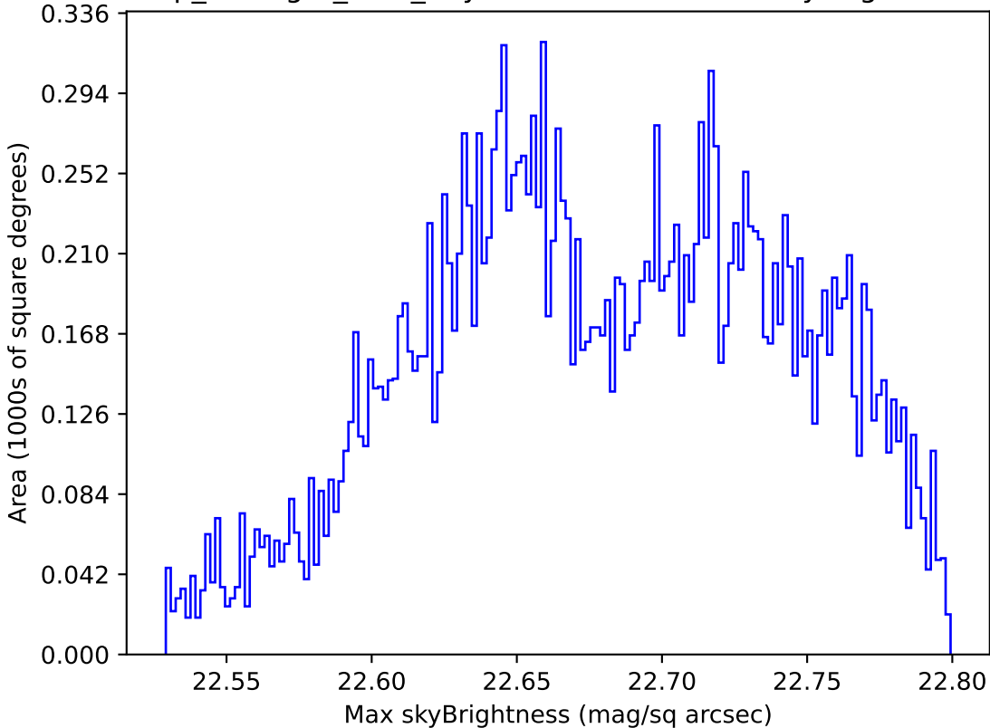
scp_reweight_v3.3_10yrs Yr 1 u band: Max skyBrightness
