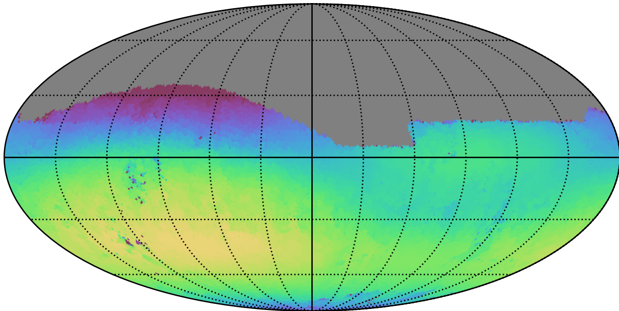
scp_reweight_v3.3_10yrs Yr 1 r band: Max skyBrightness
