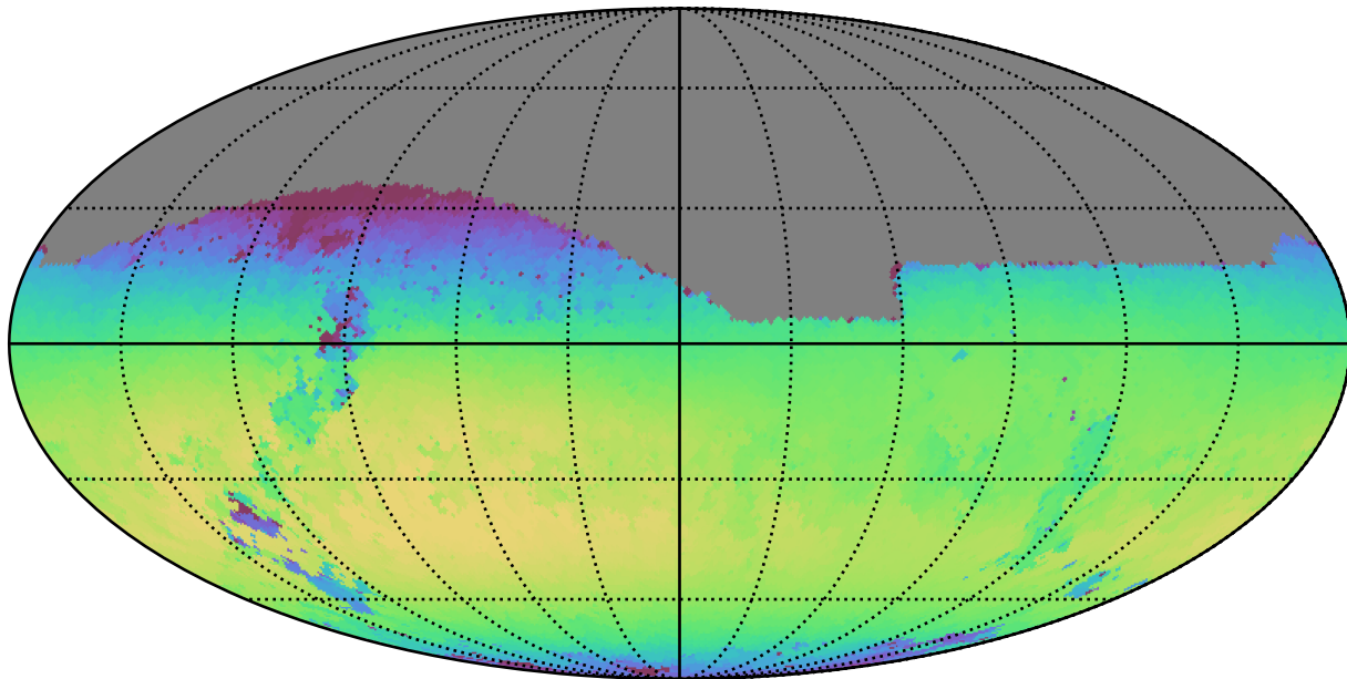
scp_reweight_v3.3_10yrs Yr 1 i band: Max skyBrightness
