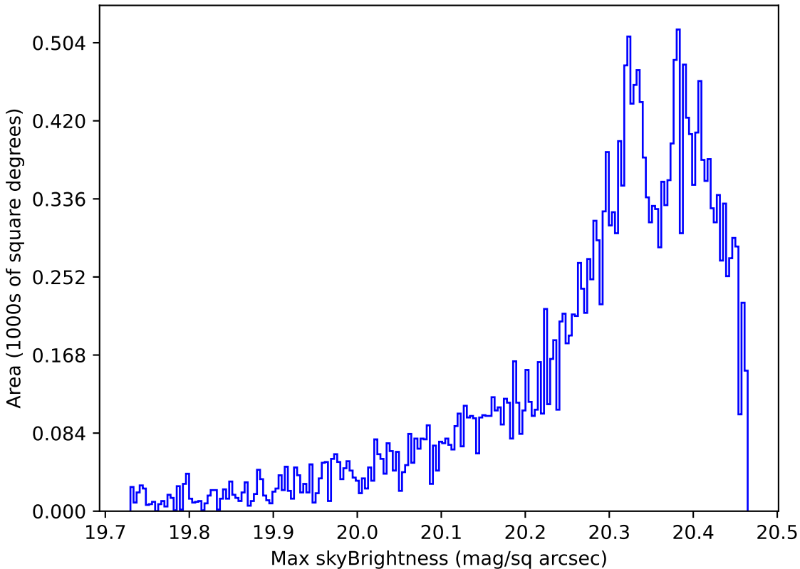
scp_reweight_v3.3_10yrs Yr 1 i band: Max skyBrightness
