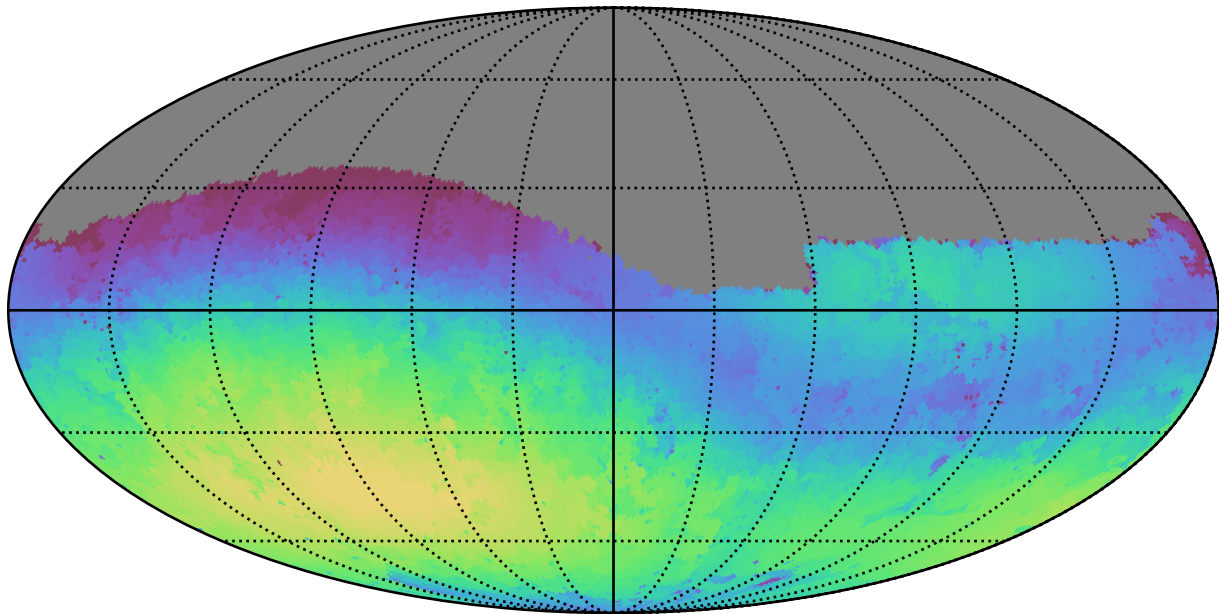
scp_reweight_v3.3_10yrs Yr 1 g band: Max skyBrightness
