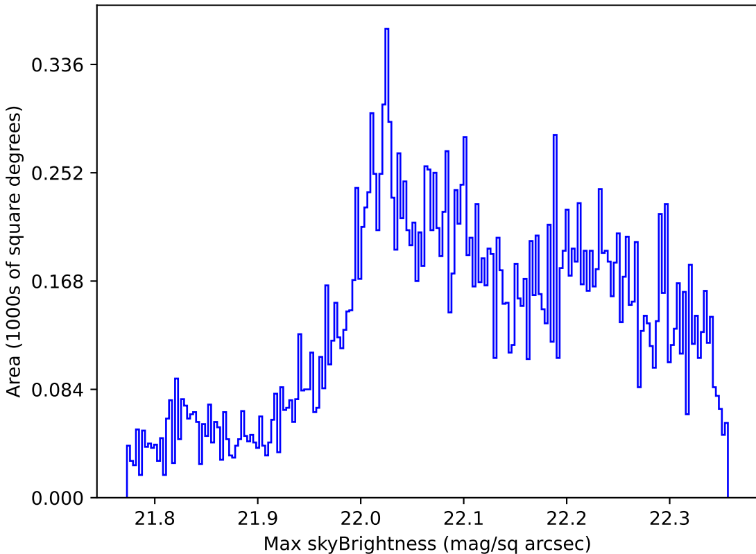
scp_reweight_v3.3_10yrs Yr 1 g band: Max skyBrightness
