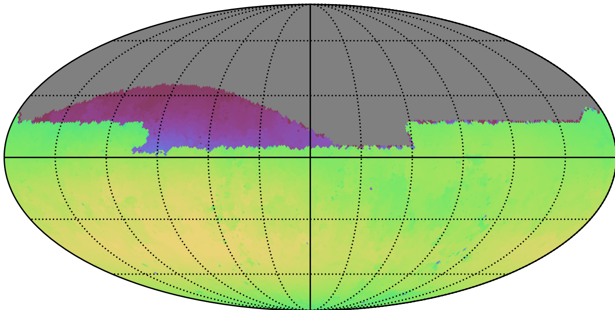
scp_reweight_v3.3_10yrs Yr 1 all bands: Max skyBrightness
