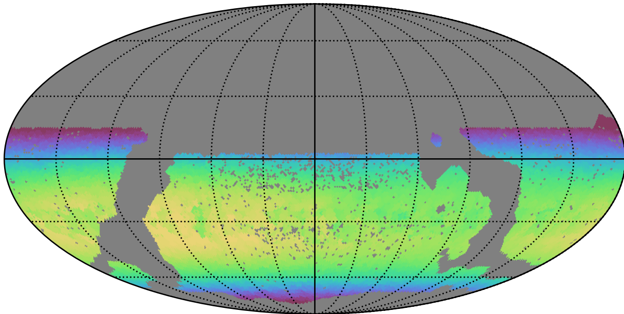
scp_reweight_v3.3_10yrs WFD z band: Max skyBrightness
