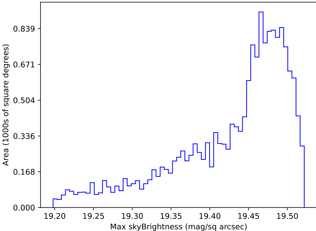
scp_reweight_v3.3_10yrs WFD z band: Max skyBrightness
