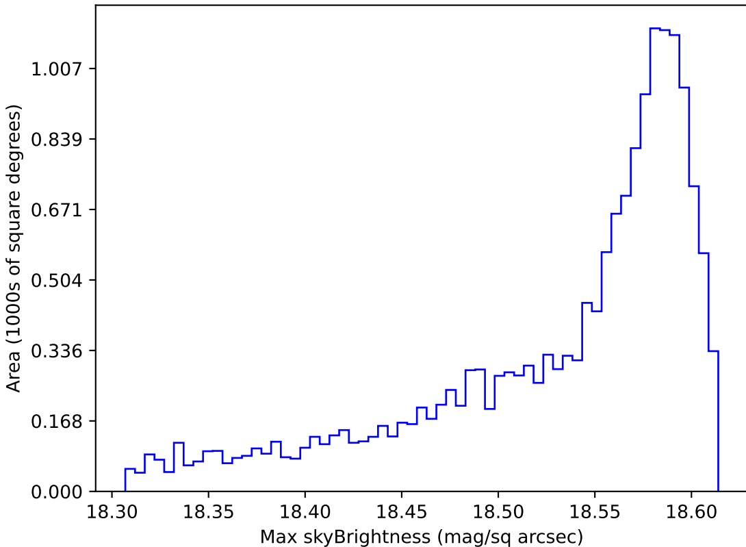
scp_reweight_v3.3_10yrs WFD y band: Max skyBrightness
