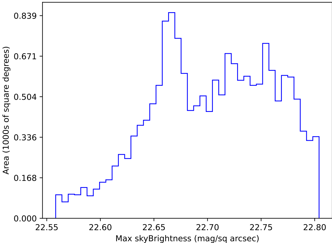
scp_reweight_v3.3_10yrs WFD u band: Max skyBrightness
