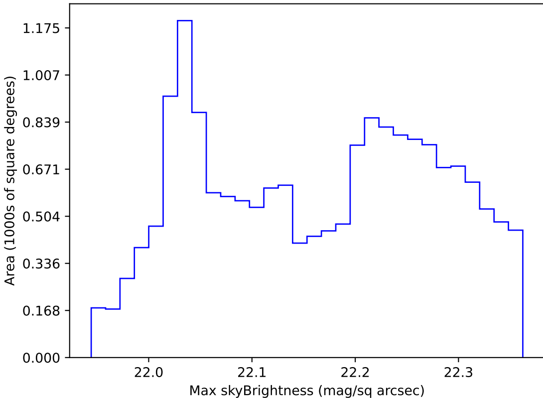
scp_reweight_v3.3_10yrs WFD g band: Max skyBrightness
