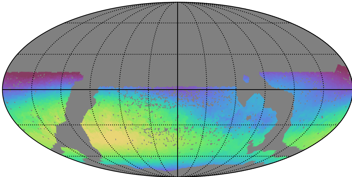
scp_reweight_v3.3_10yrs WFD all bands: Max skyBrightness
