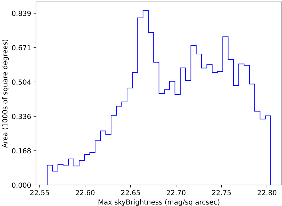
scp_reweight_v3.3_10yrs WFD all bands: Max skyBrightness
