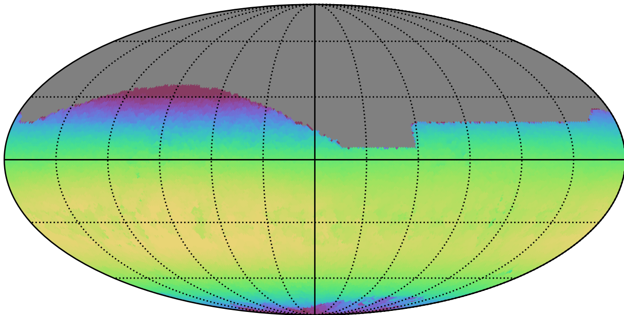
scp_reweight_v3.3_10yrs All sky z band: Max skyBrightness
