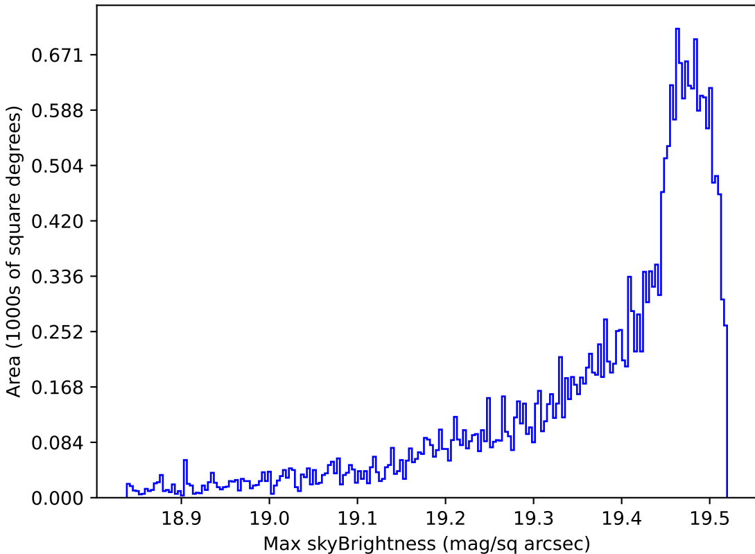
scp_reweight_v3.3_10yrs All sky z band: Max skyBrightness
