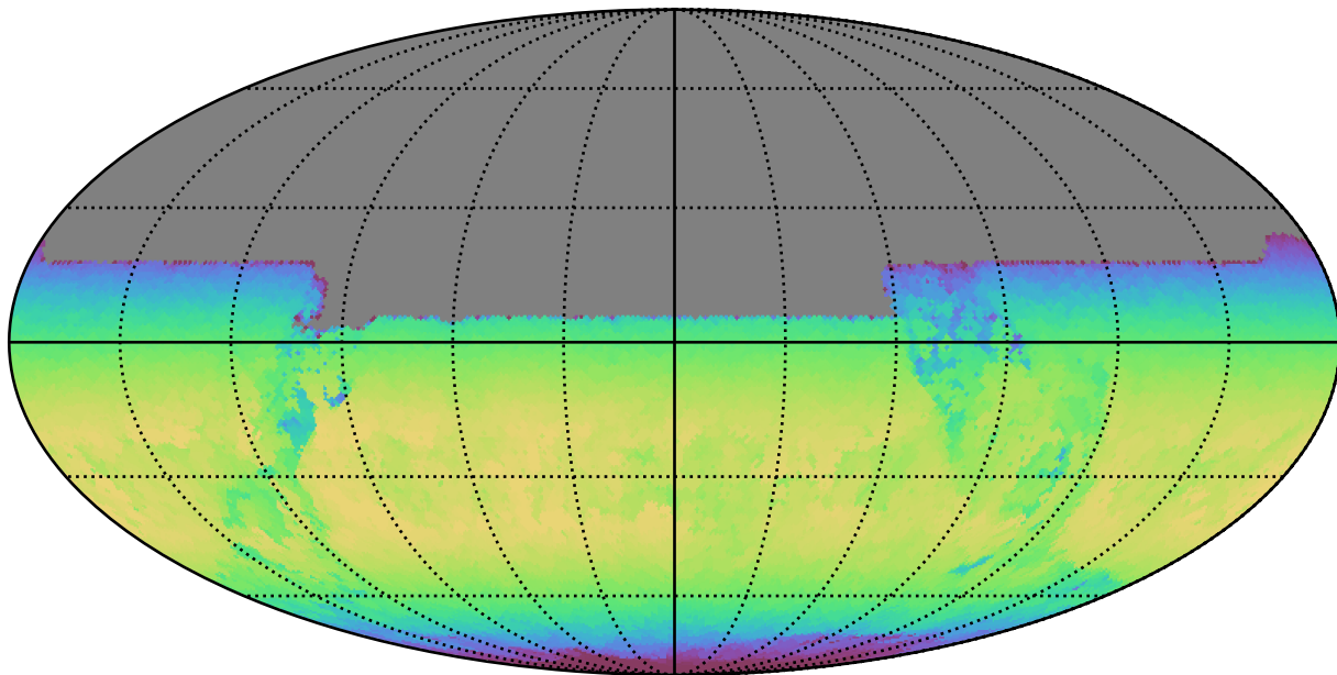
scp_reweight_v3.3_10yrs All sky y band: Max skyBrightness
