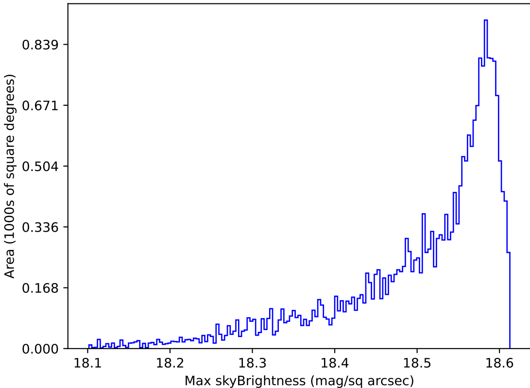
scp_reweight_v3.3_10yrs All sky y band: Max skyBrightness
