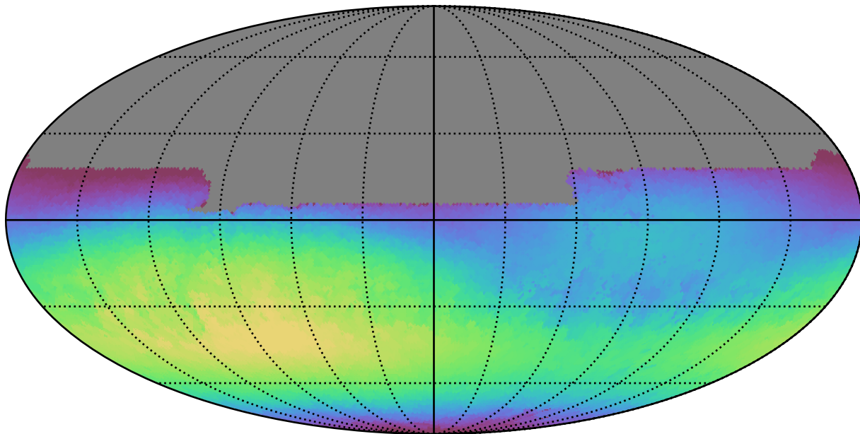
scp_reweight_v3.3_10yrs All sky u band: Max skyBrightness
