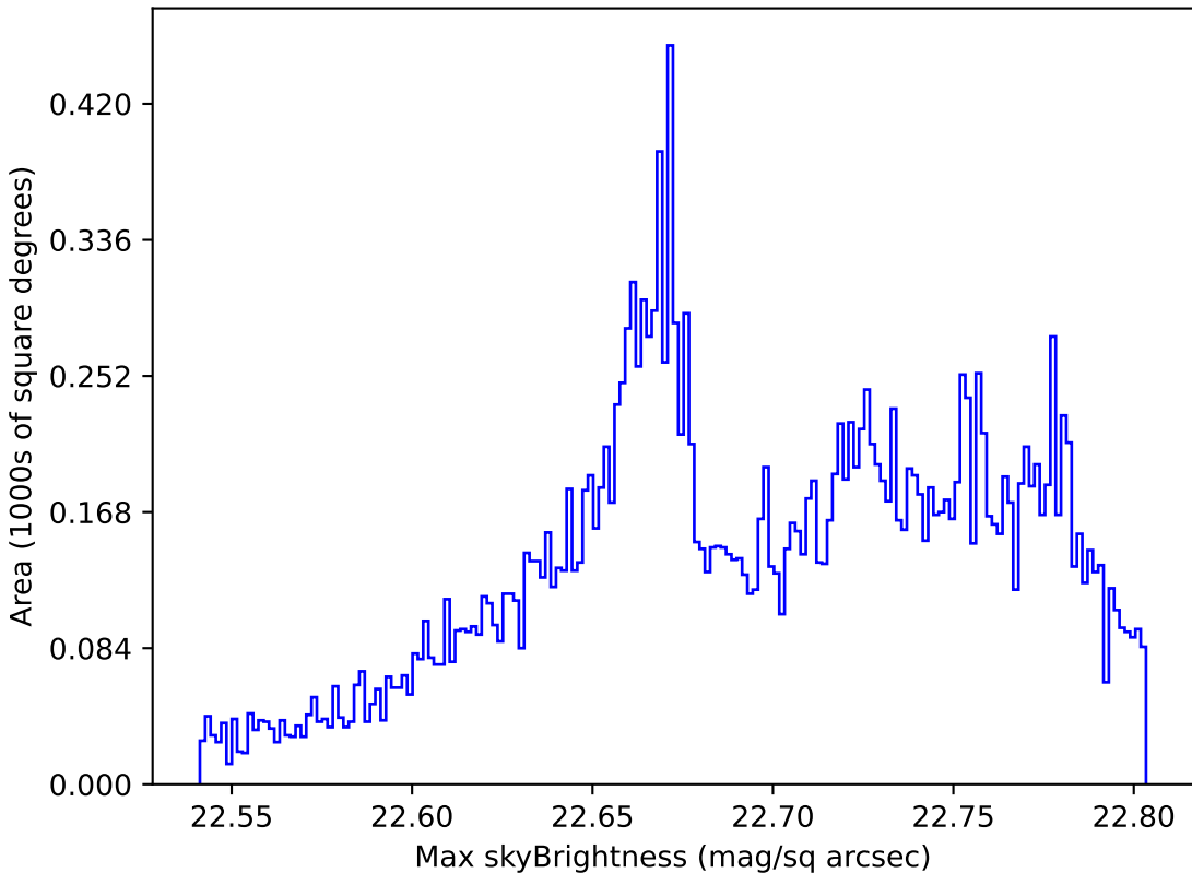
scp_reweight_v3.3_10yrs All sky u band: Max skyBrightness
