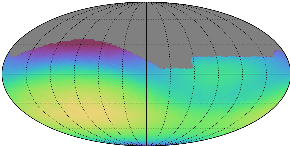
scp_reweight_v3.3_10yrs All sky r band: Max skyBrightness
