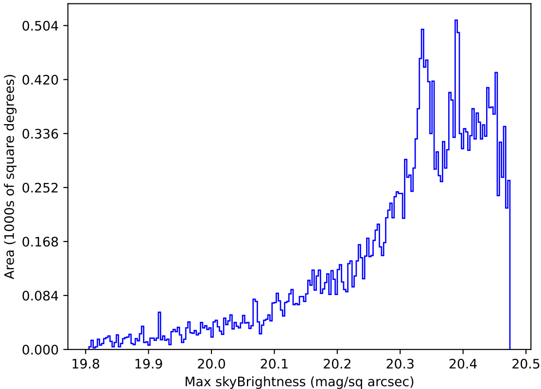
scp_reweight_v3.3_10yrs All sky i band: Max skyBrightness
