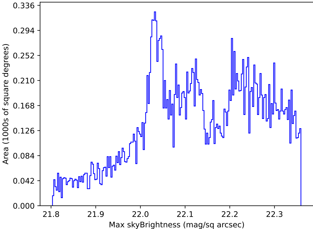
scp_reweight_v3.3_10yrs All sky g band: Max skyBrightness
