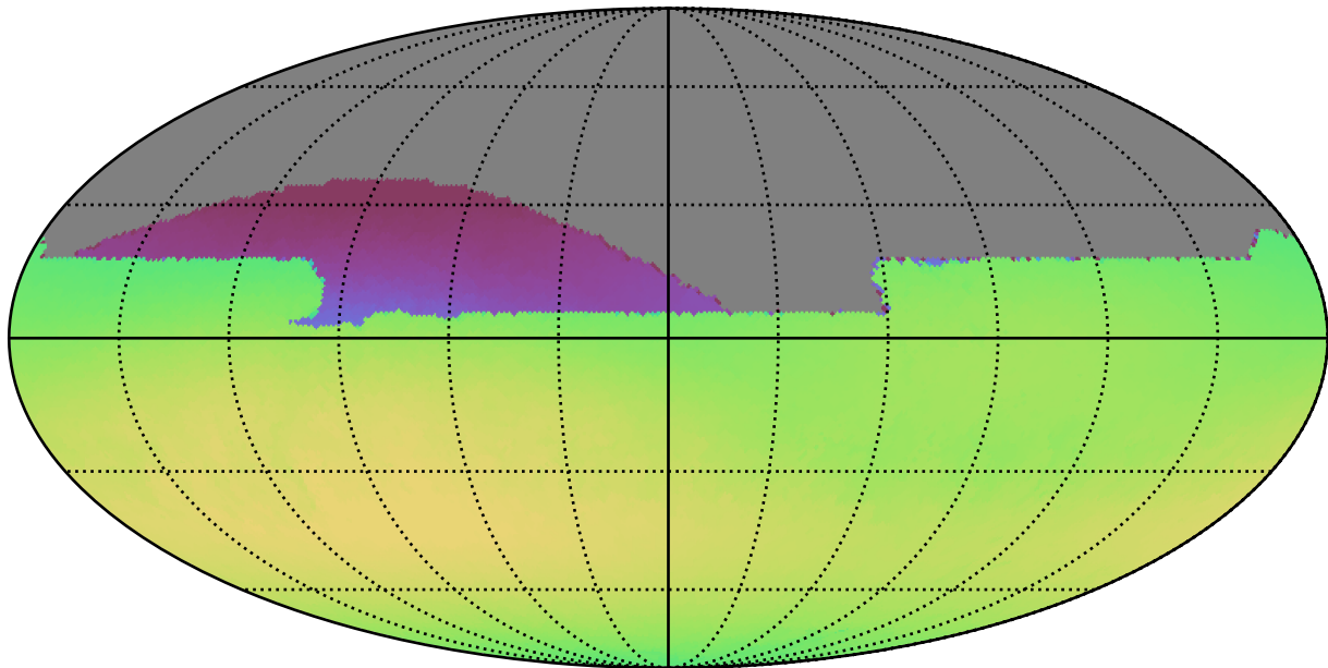
scp_reweight_v3.3_10yrs All sky all bands: Max skyBrightness
