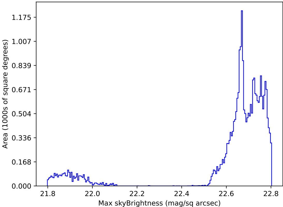
scp_reweight_v3.3_10yrs All sky all bands: Max skyBrightness
