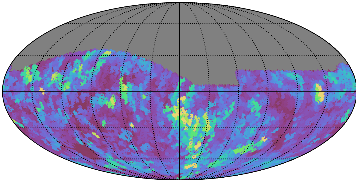
scp_reweight_v3.3_10yrs Yr 1 z band: Max seeingGeom
