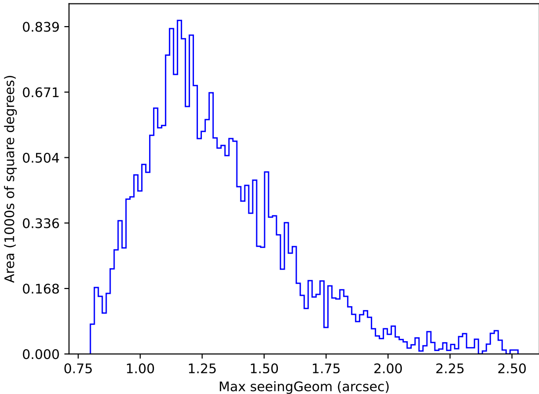
scp_reweight_v3.3_10yrs Yr 1 z band: Max seeingGeom
