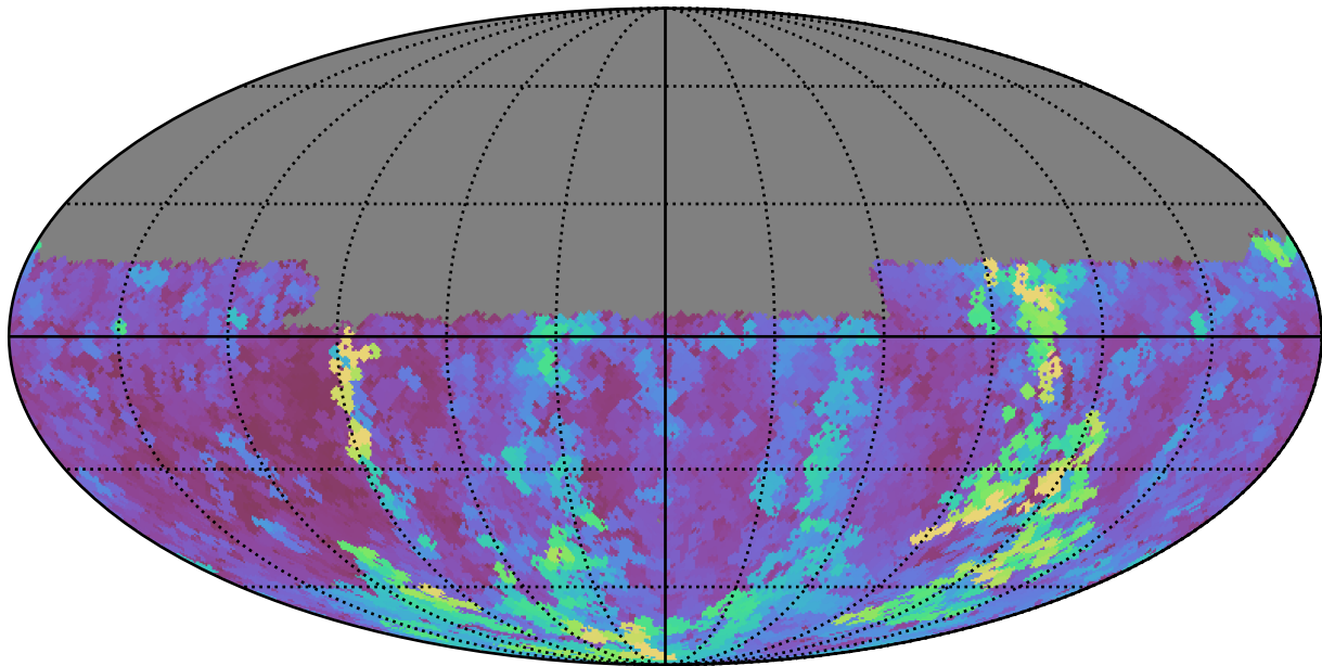
scp_reweight_v3.3_10yrs Yr 1 u band: Max seeingGeom
