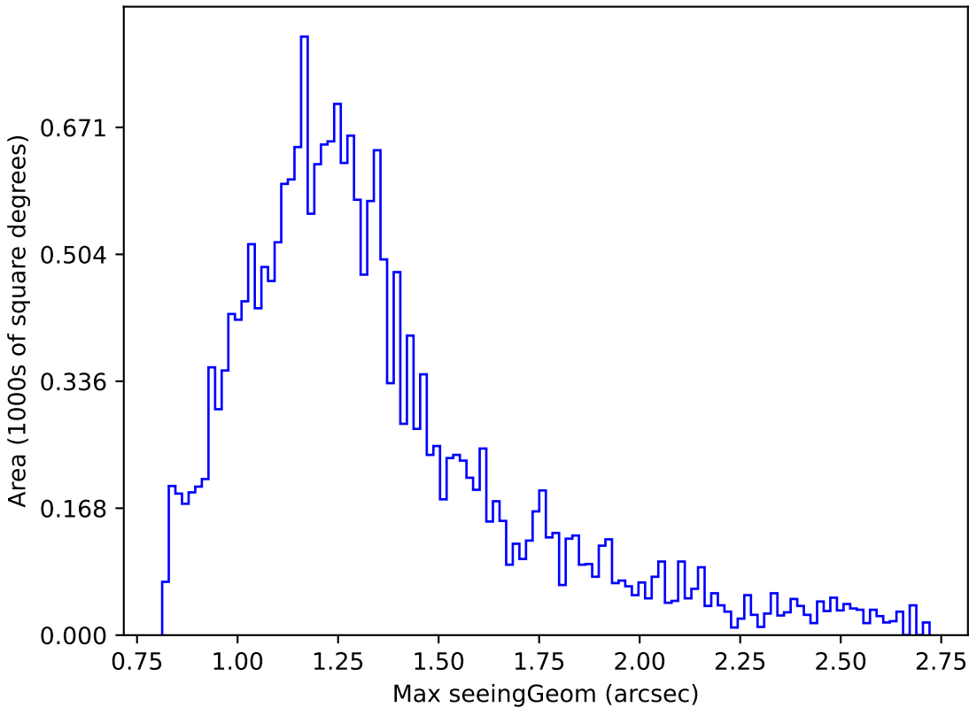
scp_reweight_v3.3_10yrs Yr 1 u band: Max seeingGeom
