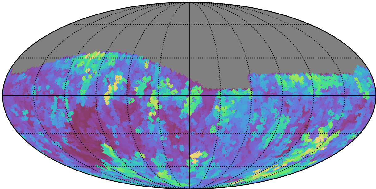
scp_reweight_v3.3_10yrs Yr1 r band: Max seeingGeom
