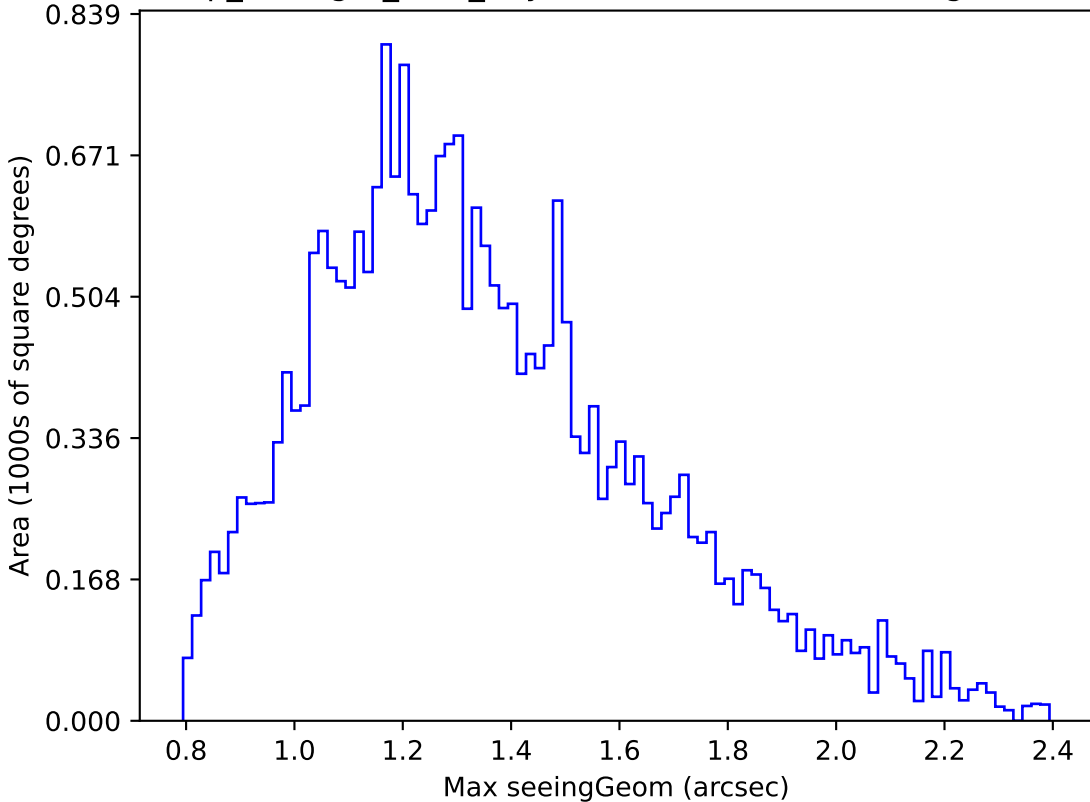
scp_reweight_v3.3_10yrs Yr 1 r band: Max seeingGeom
