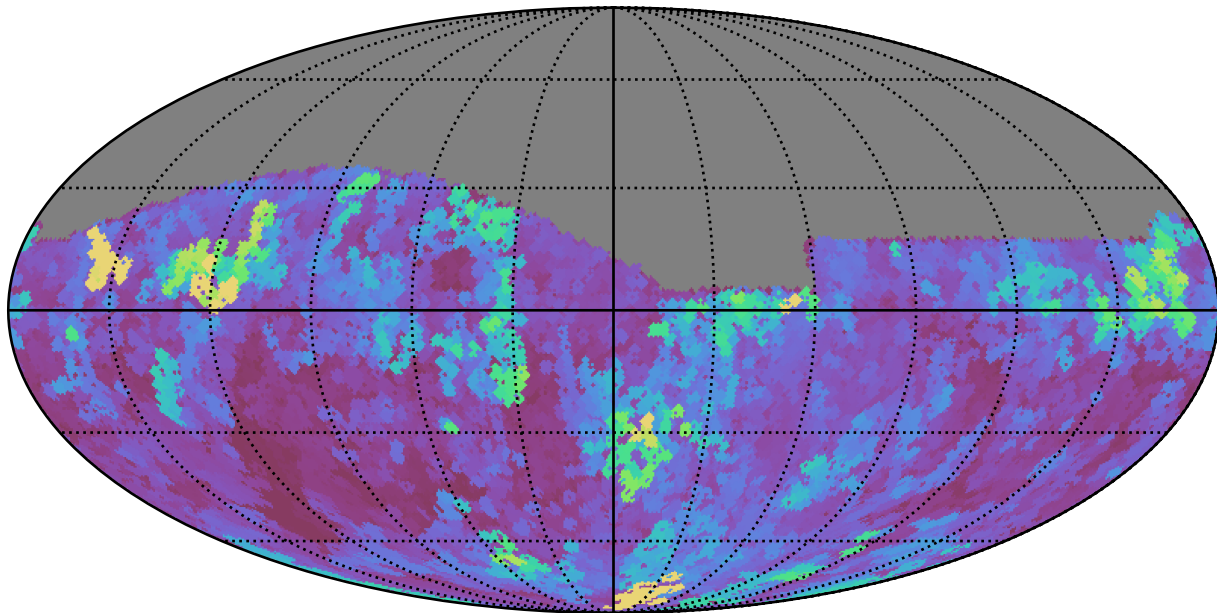
scp_reweight_v3.3_10yrs Yr 1 i band: Max seeingGeom
