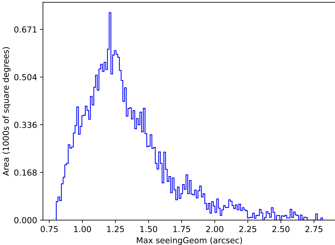
scp_reweight_v3.3_10yrs Yr 1 i band: Max seeingGeom
