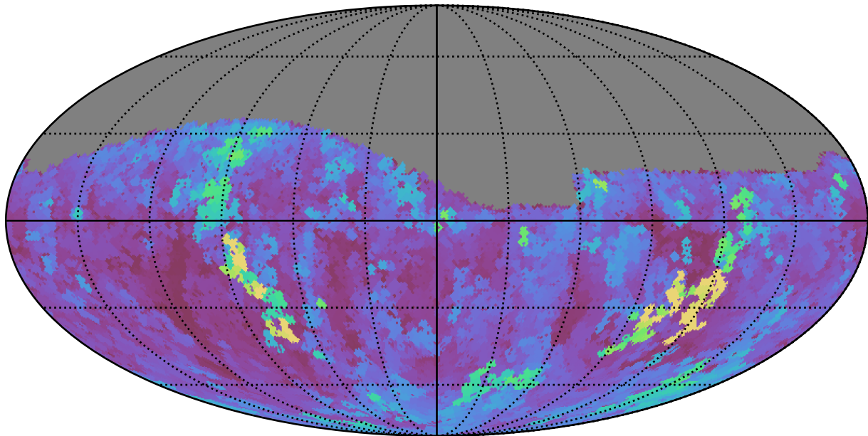
scp_reweight_v3.3_10yrs Yr 1 g band: Max seeingGeom
