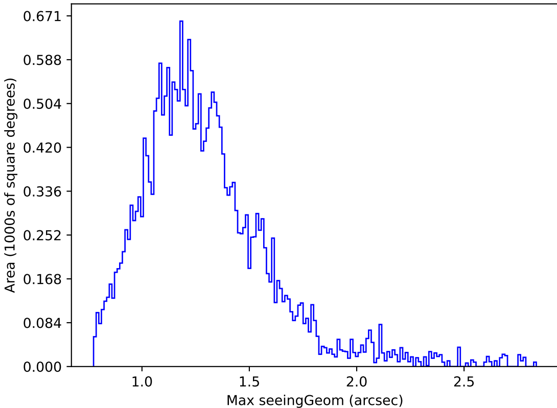
scp_reweight_v3.3_10yrs Yr 1 g band: Max seeingGeom
