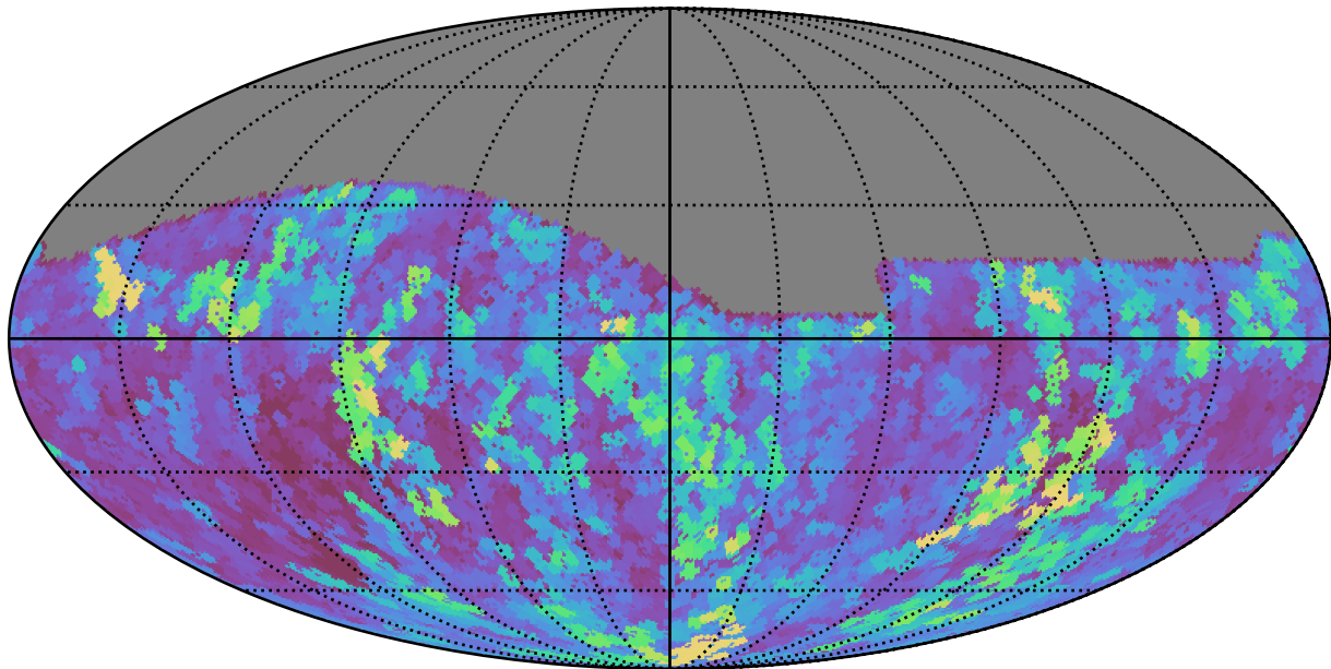
scp_reweight_v3.3_10yrs Yr 1 all bands: Max seeingGeom
